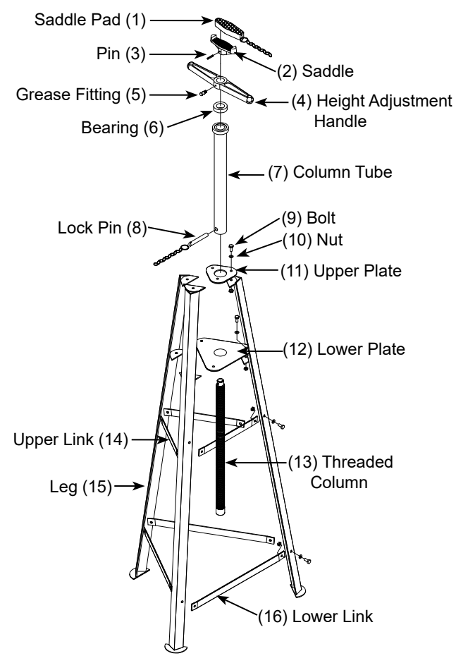
Figure 1 - Model 33020 Components
