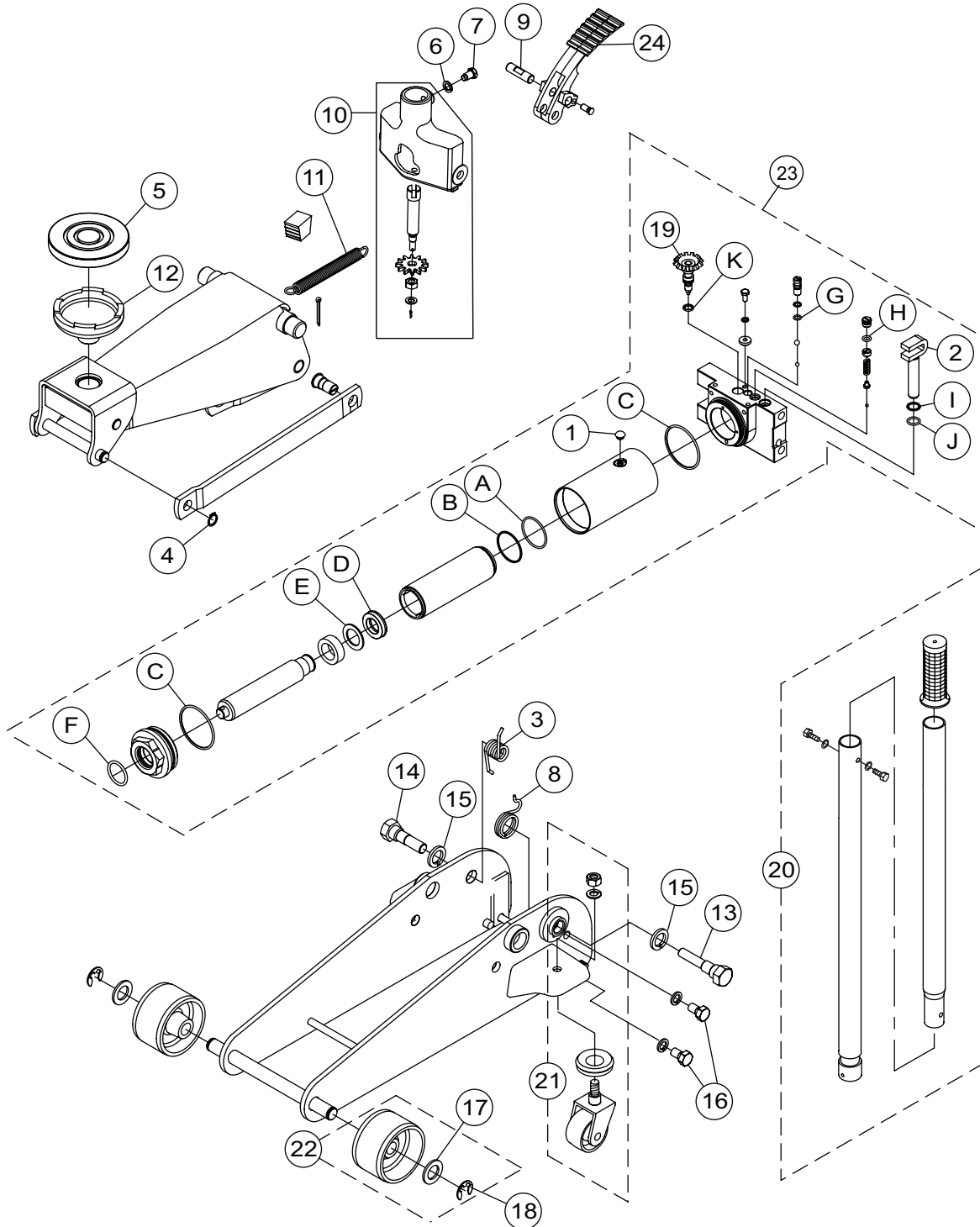
Figure 2 - Replacement Parts Illustration for Model BH6034B
