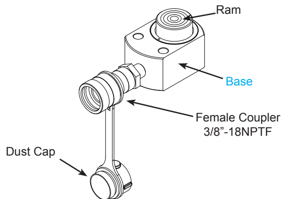
Figure 1 - Typical Flat Body Cylinder Components
