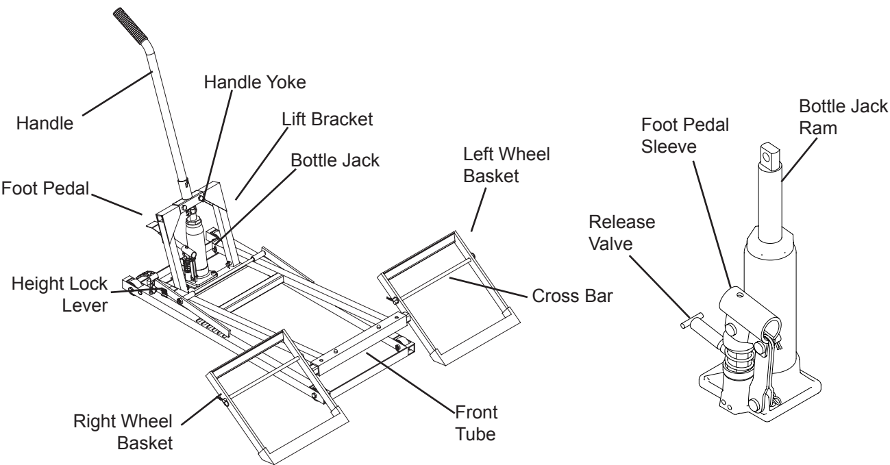
Figure 1: Lawn Mower Lift nomenclature.
